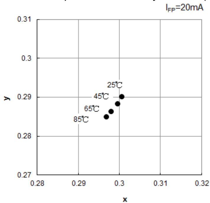
Ambient Temperature vs. Chromaticity Coordinate ( I_{FP}=20\text{mA} )
