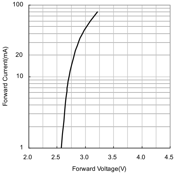
Forward Voltage vs. Forward Current (Ta=25°C)
