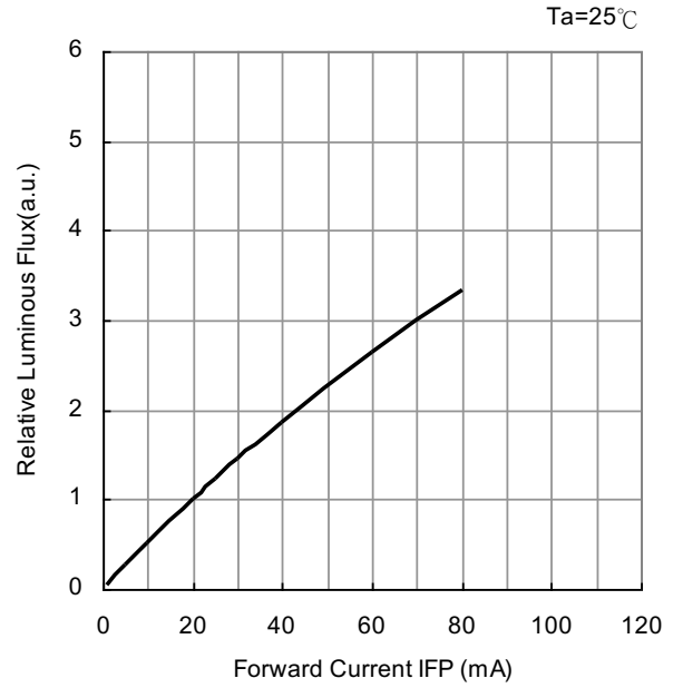
Forward Current vs. Relative Luminous Flux (Ta=25°C)
