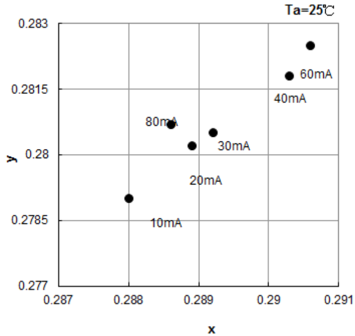
Forward Current vs. Chromaticity Coordinate ( T_A=25^\circ\text{C} )
