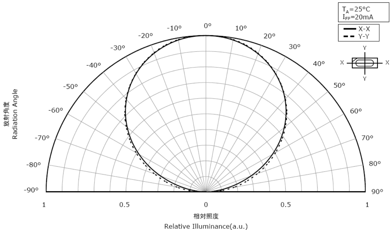
Radiation Pattern( T_A=25^{\circ}\text{C} , I_{FP}=20\text{mA} )
