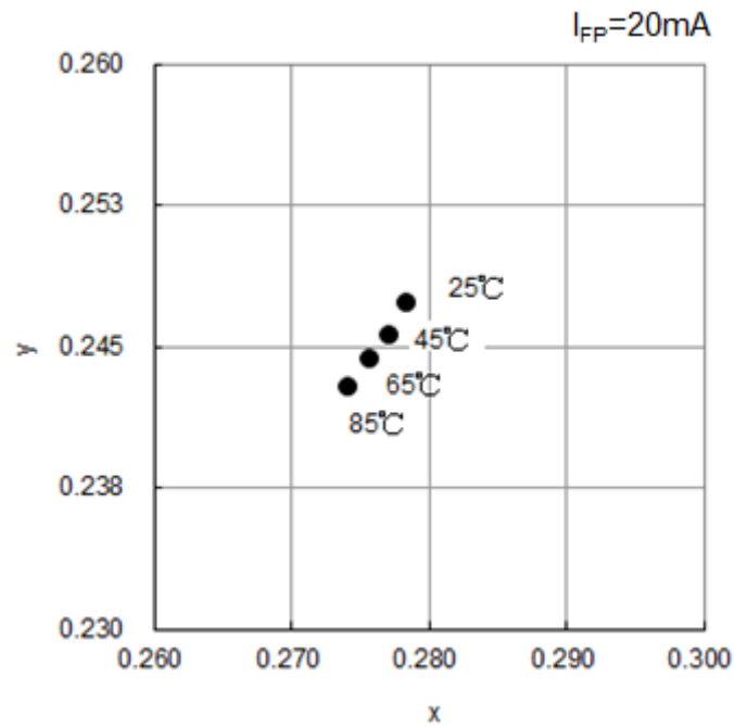
Ambient Temperature vs. Chromaticity Coordinate ( I_{FP}=20\text{mA} )
